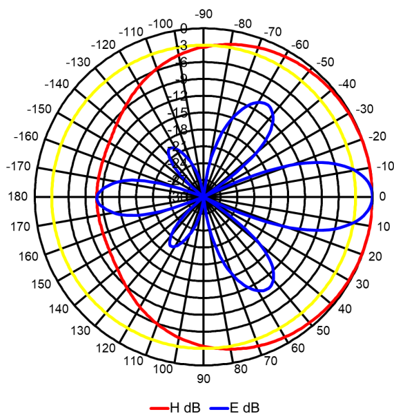
RADIATION PATTERN
